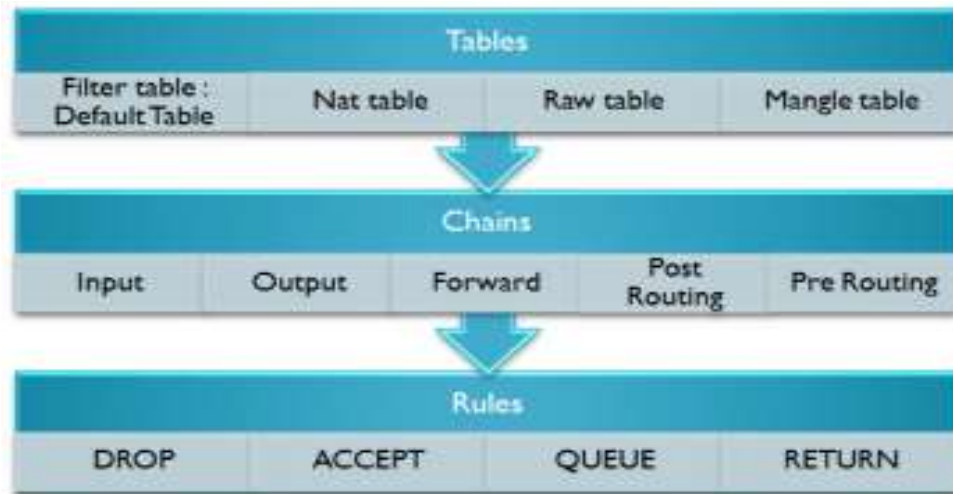
Figure 2.4 Iptables Architecture
